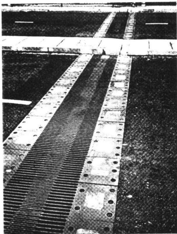
When the parts of a bridge-deck expand, the steel edges move towards each other.
