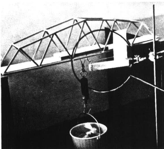
The PLON-bridge loaded. The bending gauge is clearly visible in the enlarged photograph.
