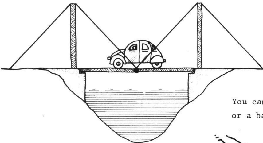
A stayed girder bridge: the bridge-deck doesn't bend much, because the stays carry part of the car's weight.
