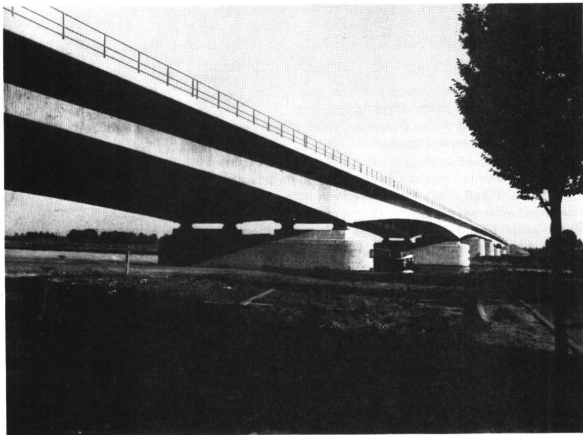
The bridge at Wessem under construction (above) and completed (below). By choosing the right building scheme, materials and shape, the engineers have succeeded in constructing a strong bridge without causing too much hindrance to ship traffic. The bridge consists of prestressed concrete sections (see Reading Text 2, ) and is constructed using the "cantilever" method. The photograph above clearly shows the concrete "tubes" supporting the bridge-deck from below.
