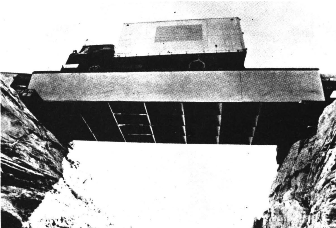
A bridge made from paper and glue only! It is about 10 m long and 5 m wide; it can hold a 4-ton lorry. Its own weight is 200 kgs.
