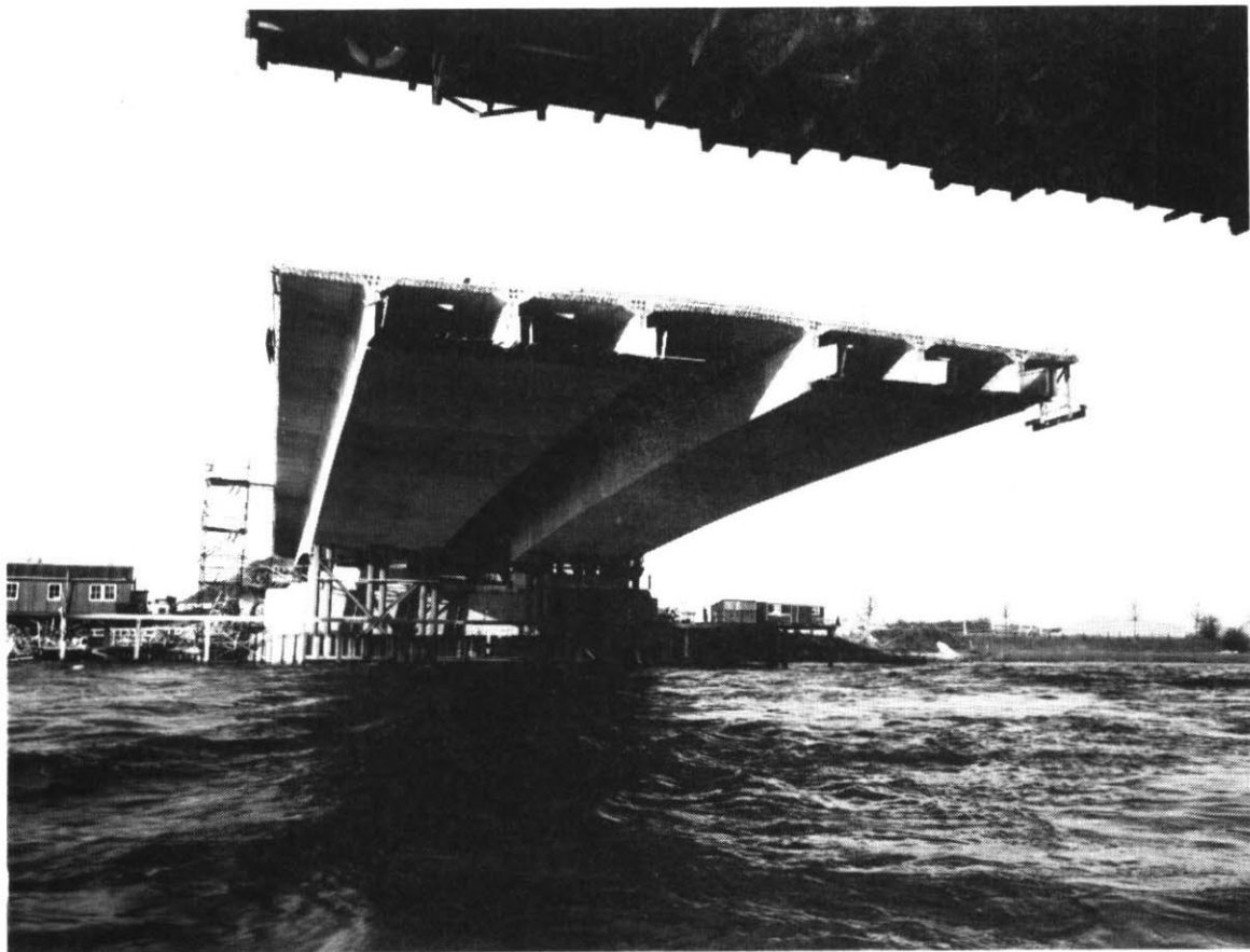
The bridge at Wessem under construction (above) and completed (below). By choosing the right building scheme, materials and shape, the engineers have succeeded in constructing a strong bridge without causing too much hindrance to ship traffic. The bridge consists of prestressed concrete sections (see Reading Text 2, ) and is constructed using the "cantilever" method. The photograph above clearly shows the concrete "tubes" supporting the bridge-deck from below.
