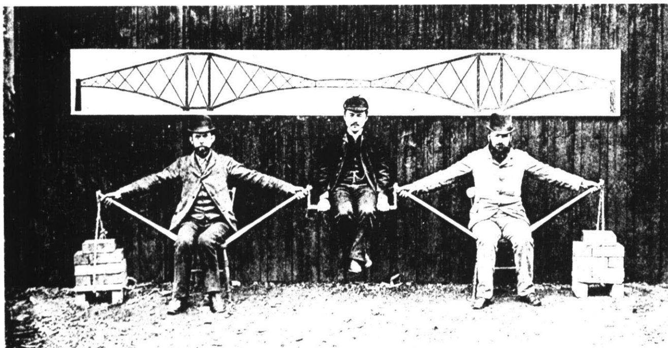
A living model of the Forth Bridge
