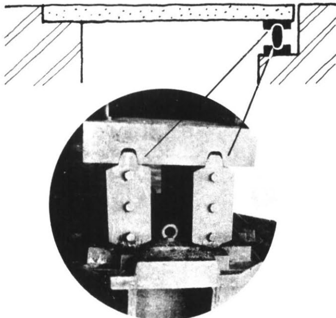
When the bridge expands (i.e. when the temperature rises), the hinges or rollers move along with the expanding deck.
